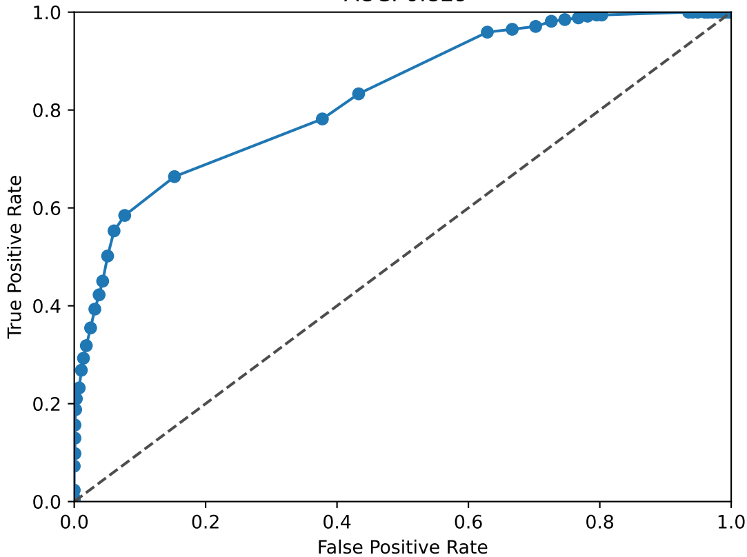
JUNB ROC Curve AUC: 0.829
