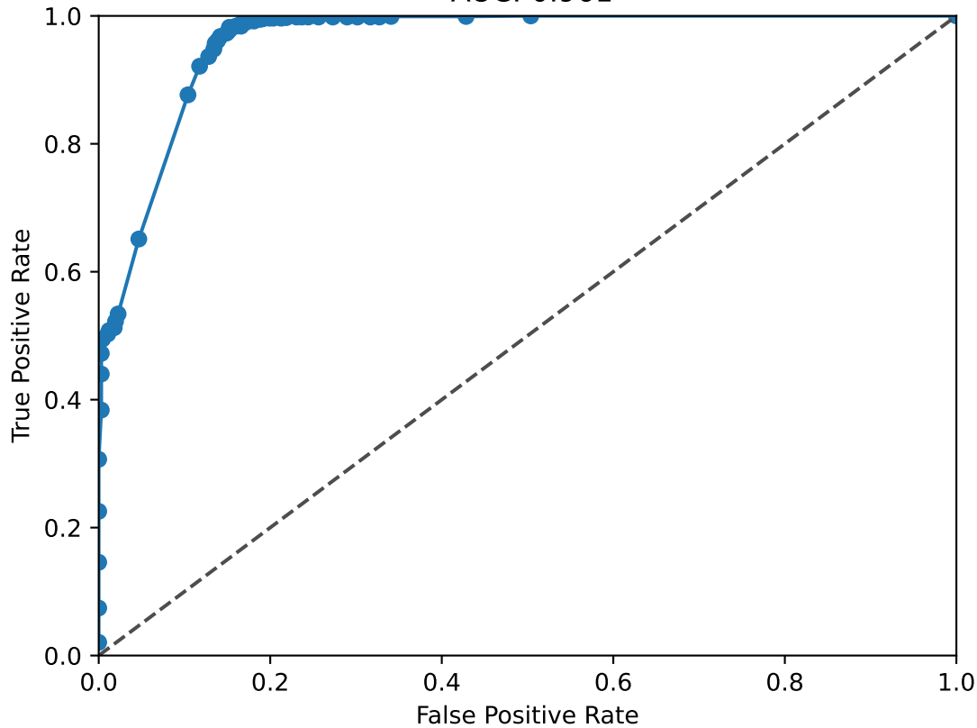
KMT2A ROC Curve AUC: 0.961
