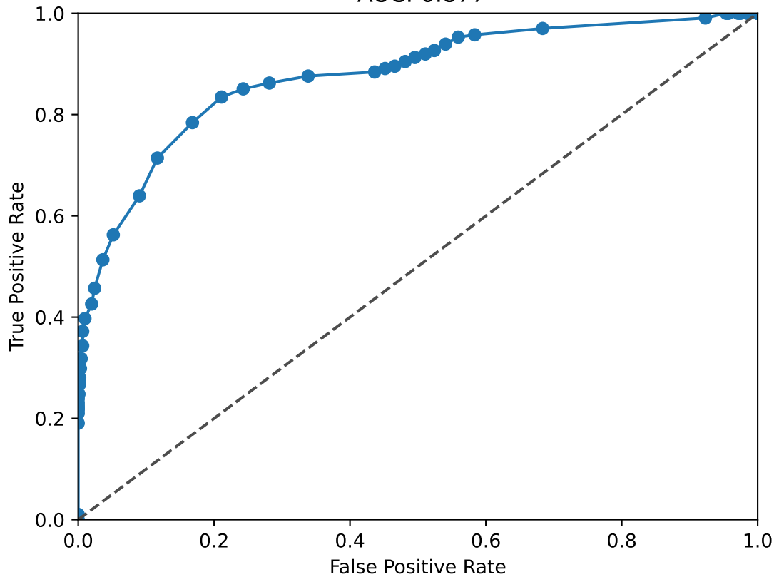
PBX1 ROC Curve AUC: 0.877
