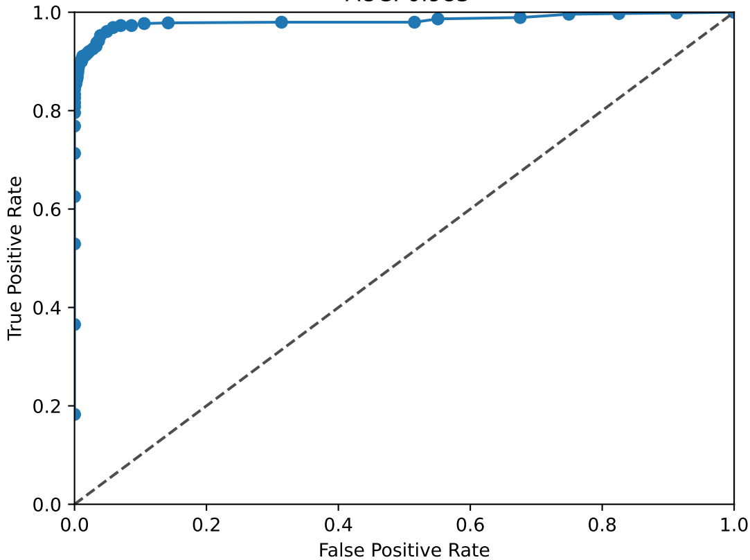
PKNOX2 ROC Curve AUC: 0.983
