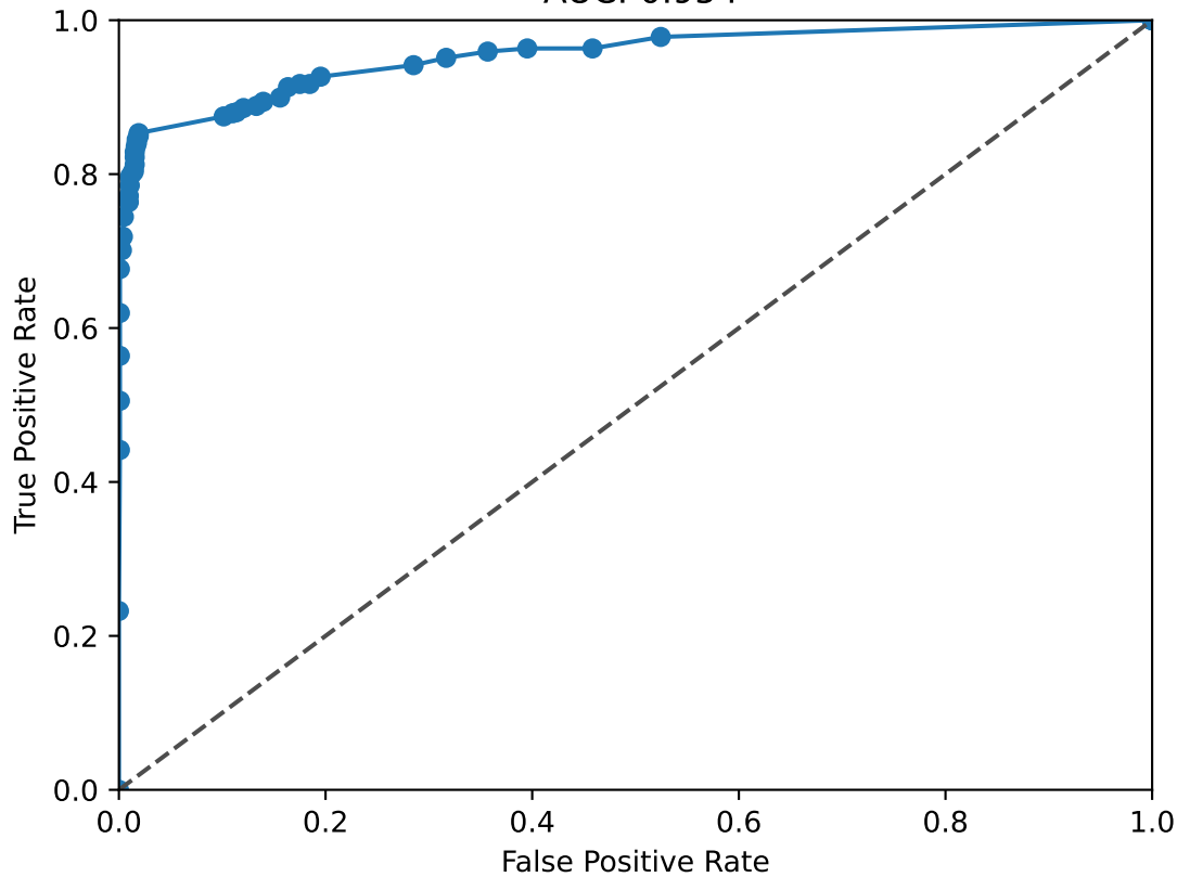
SOX11 ROC Curve AUC: 0.954
