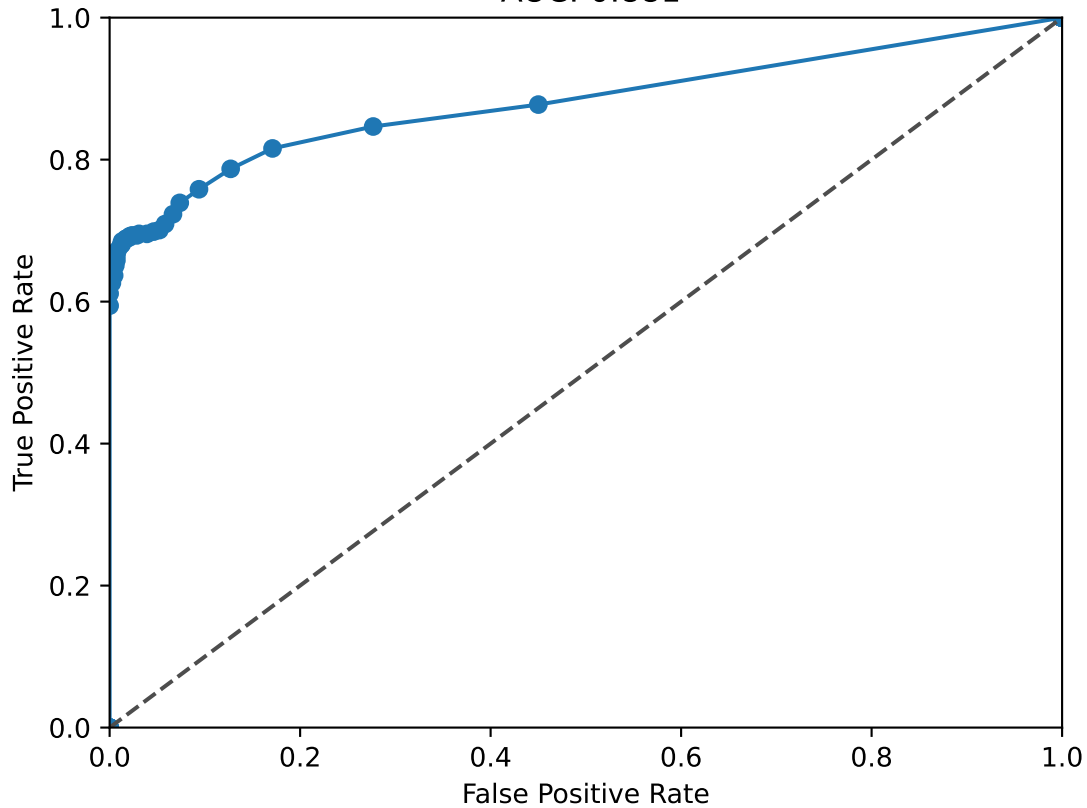
THR B ROC Curve AUC: 0.881
