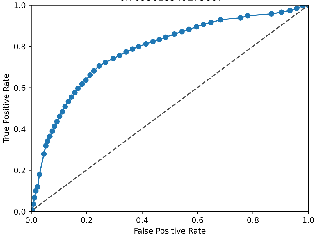
ROC Curve Data 0.7693618549275867
