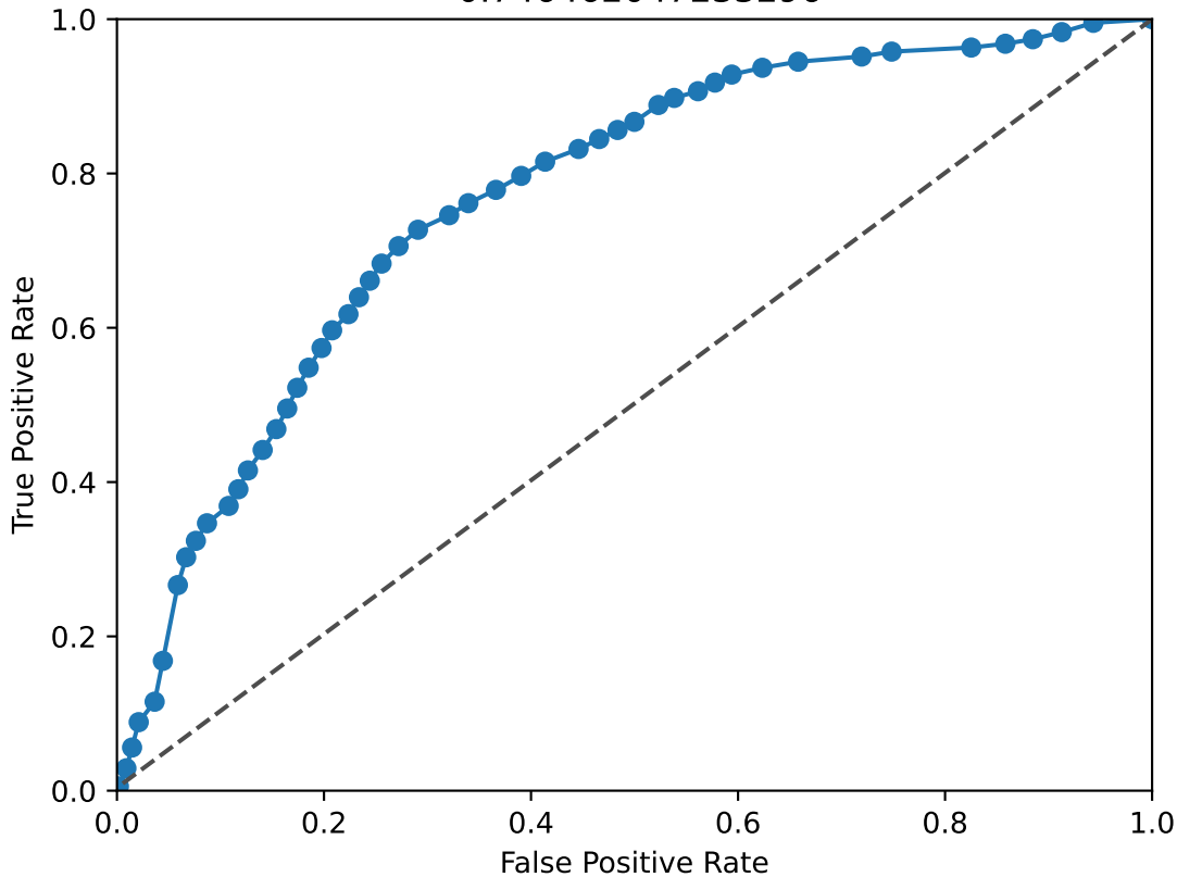
ROC Curve Data 0.746462047233296
