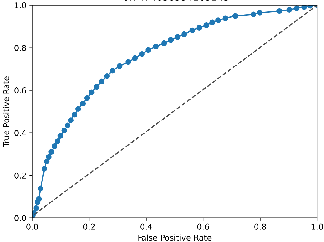
ROC Curve Data 0.7474638534169243
