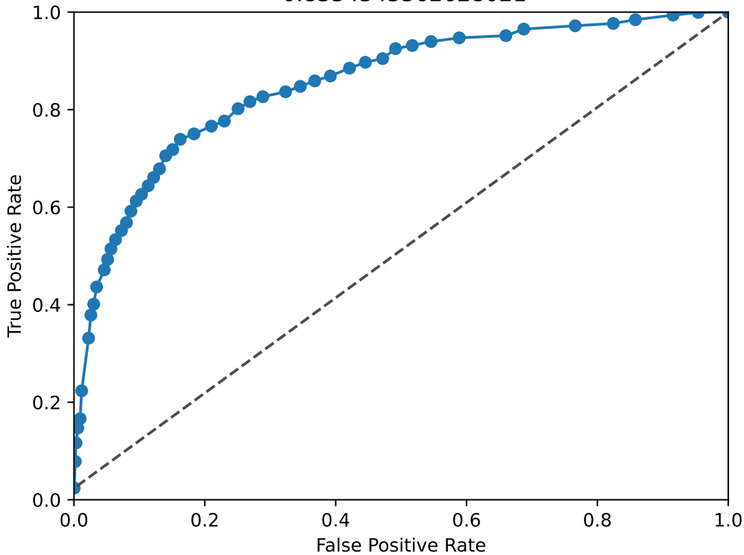
ROC Curve Data 0.8334343362628021
