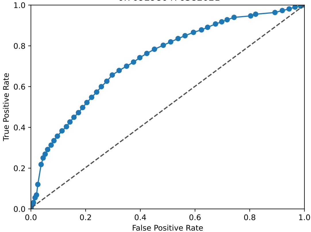
ROC Curve Data 0.7092980476382021
