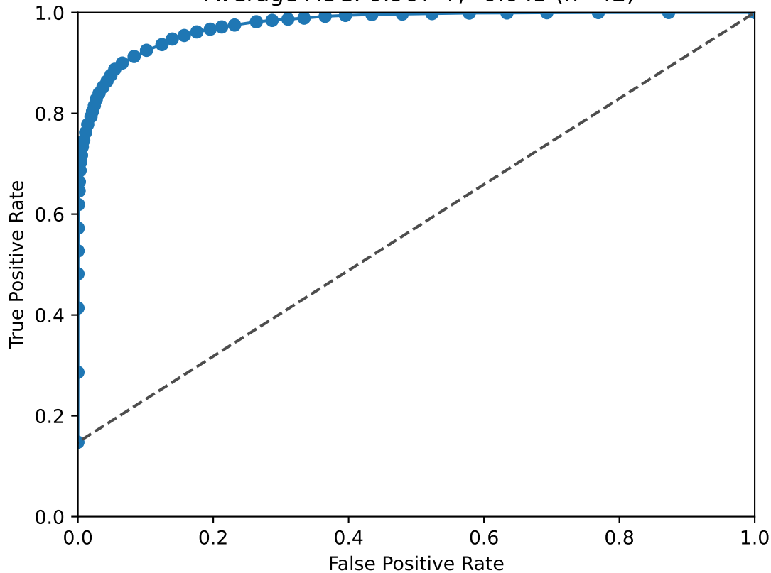
ROC Curve Data Average AUC: 0.967 \pm 0.043 (n=42)
