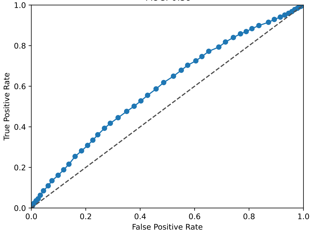
CUX2 ROC Curve AUC: 0.59
