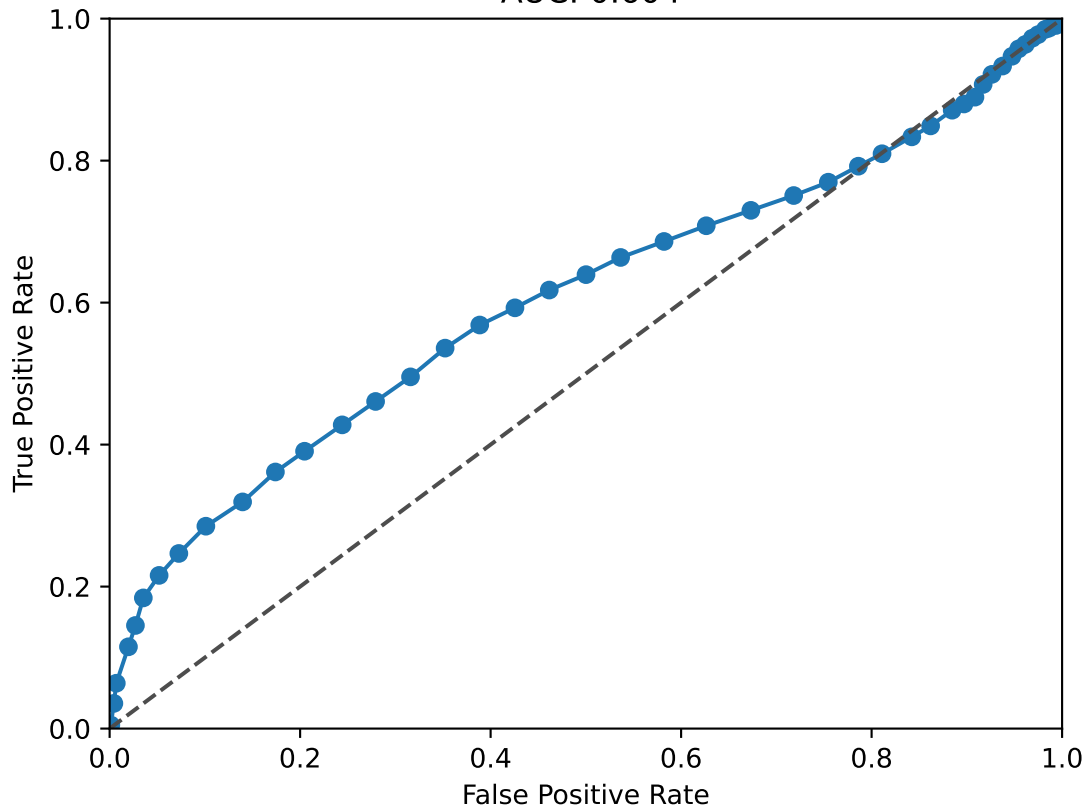
EGR1 ROC Curve AUC: 0.604
