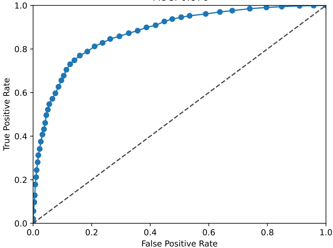
FOS ROC Curve AUC: 0.876
