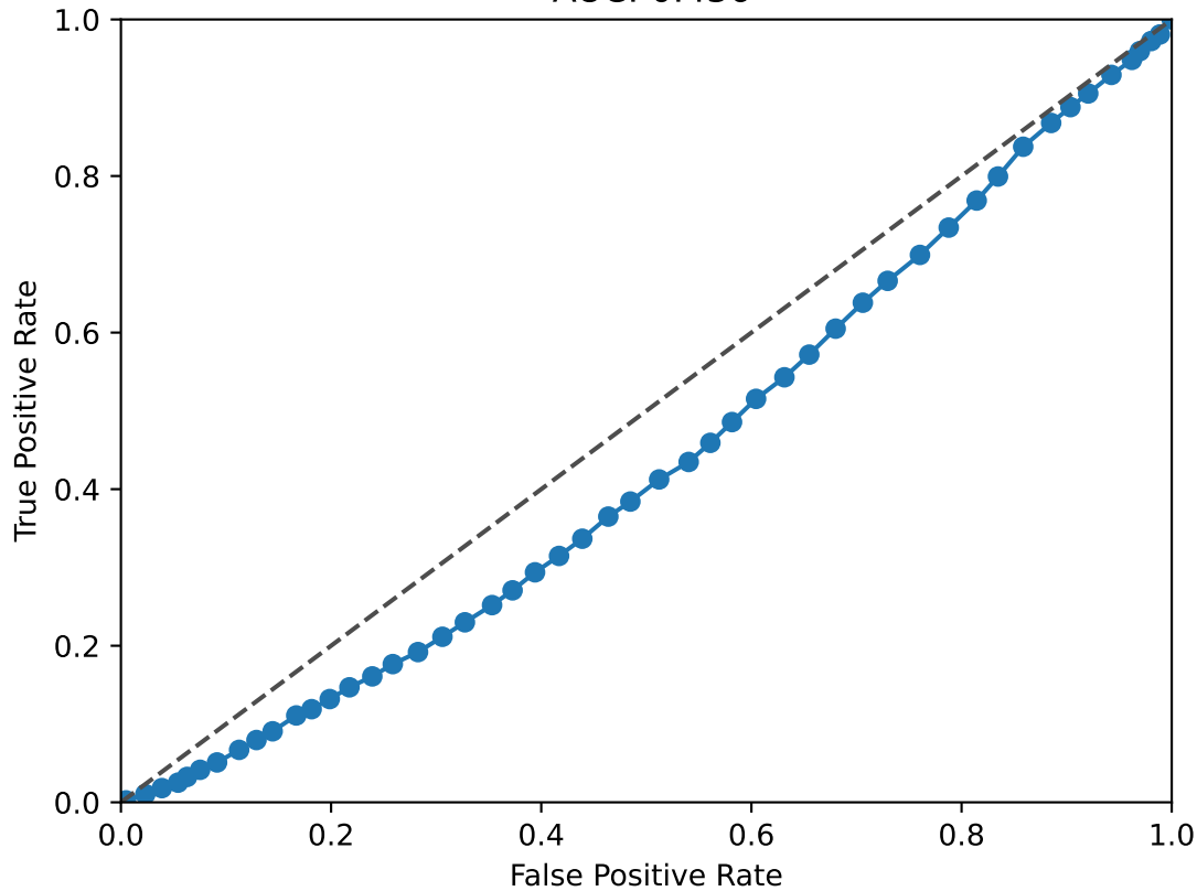
NCAM1 ROC Curve AUC: 0.436
