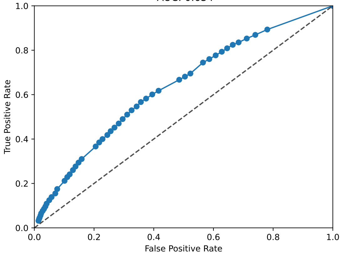
REST ROC Curve AUC: 0.634
