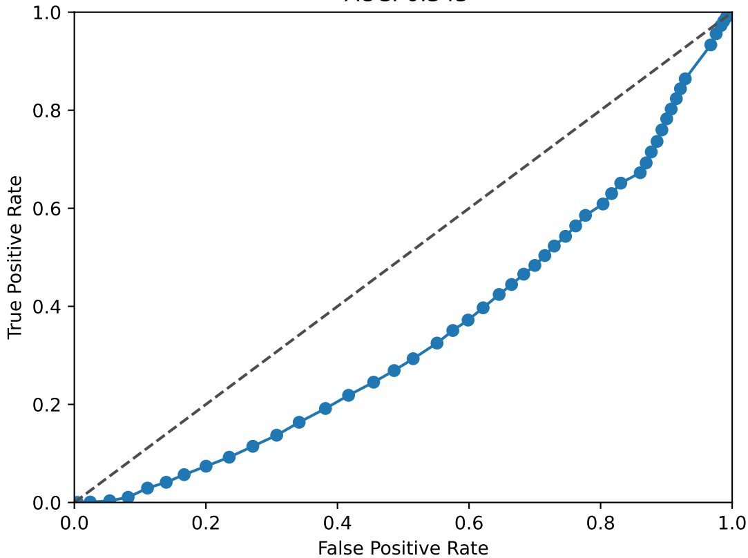
EPCAM ROC Curve AUC: 0.345
