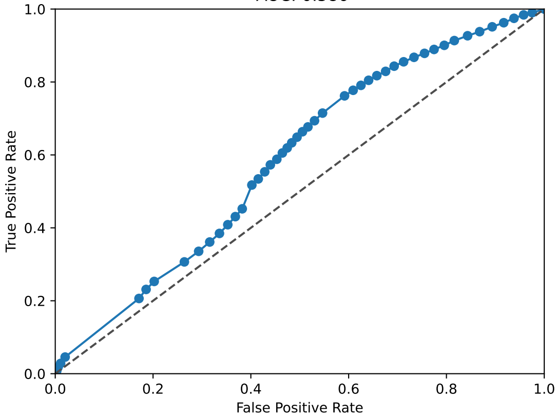
FOXO3 ROC Curve AUC: 0.586
