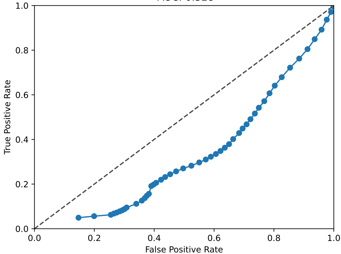
HES1 ROC Curve AUC: 0.328
