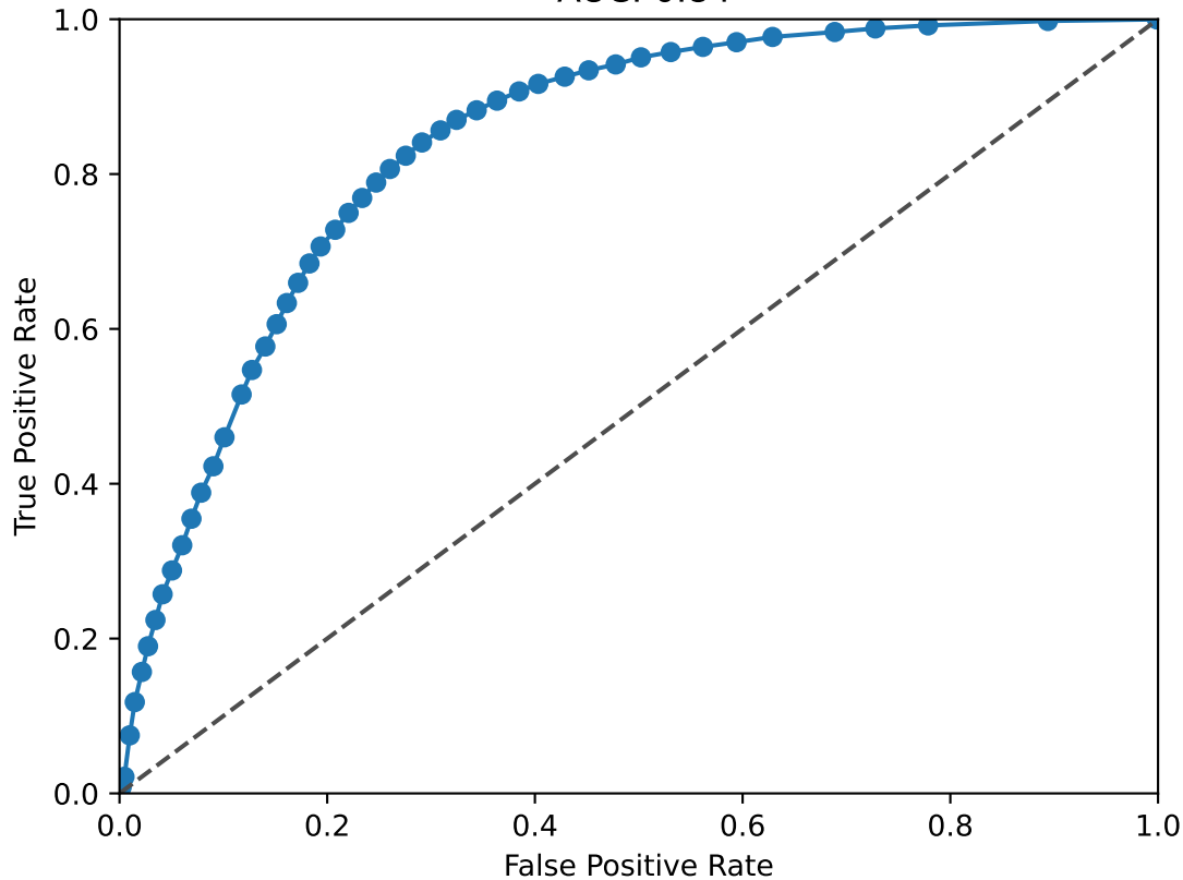
HSF2 ROC Curve AUC: 0.84
