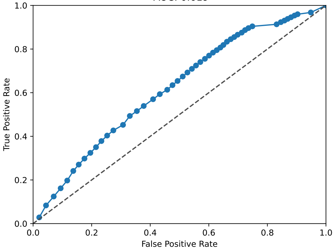
RORA_RORB ROC Curve AUC: 0.619
