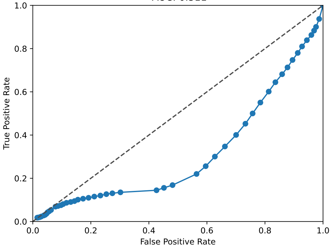
NFIX ROC Curve AUC: 0.311
