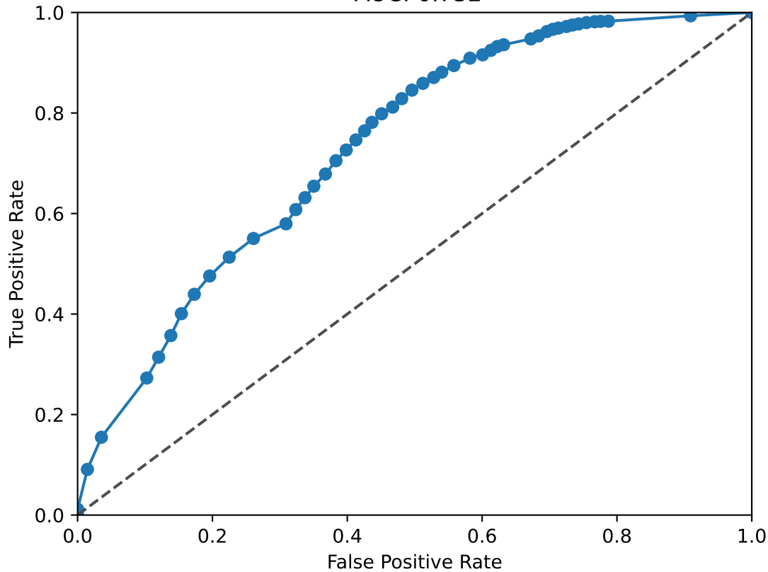
NFKB1 ROC Curve AUC: 0.732
