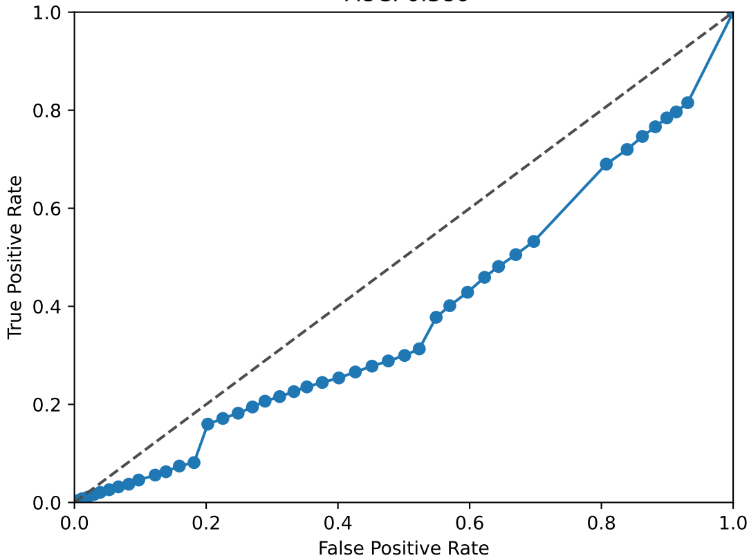
SOX11 ROC Curve AUC: 0.386
