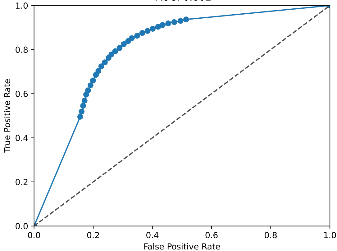
THR B ROC Curve AUC: 0.802
