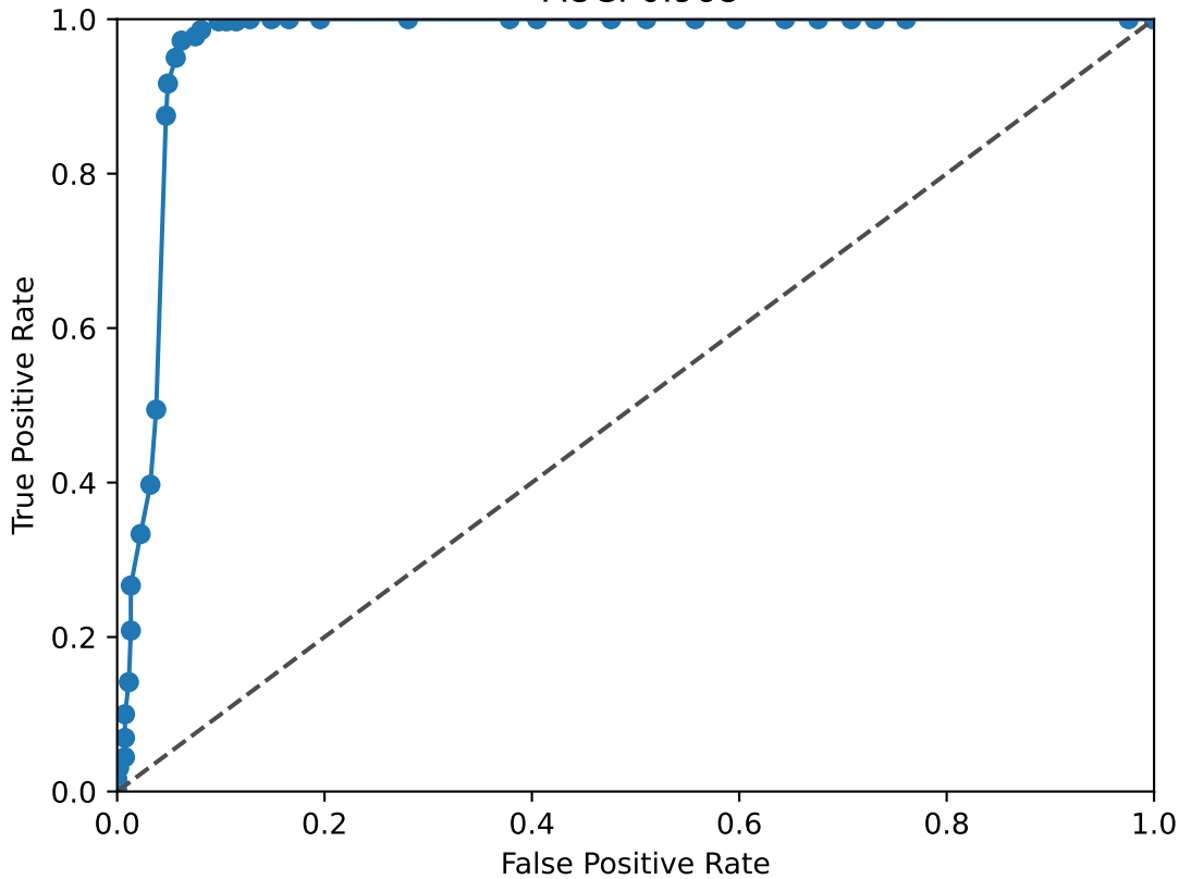
EPCAM ROC Curve AUC: 0.968
