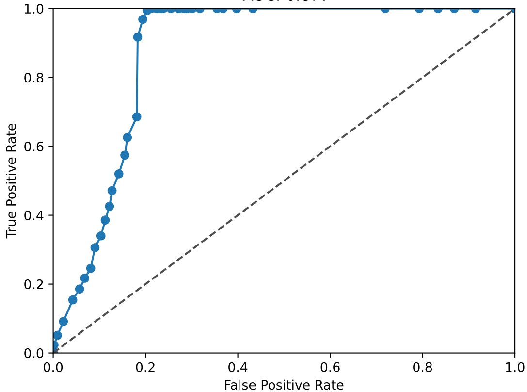
ETS1 ROC Curve AUC: 0.877
