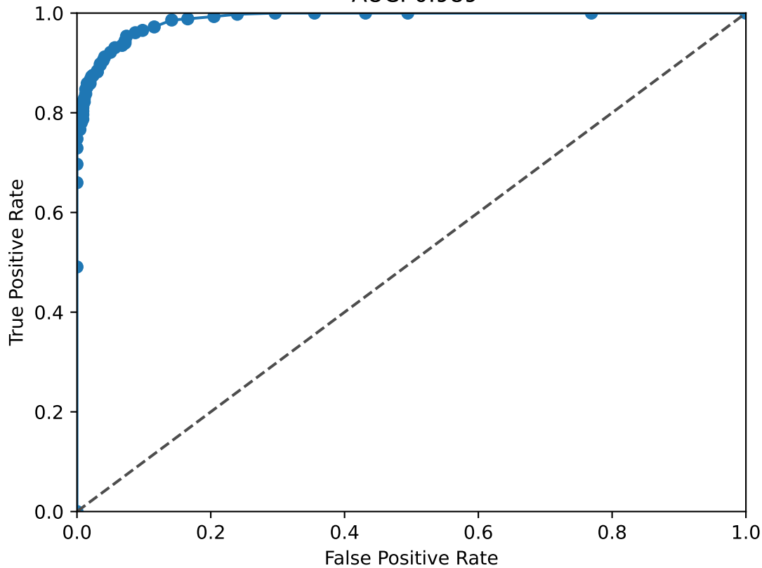
GRHL2 ROC Curve AUC: 0.989
