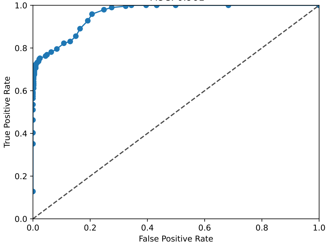
HSF2 ROC Curve AUC: 0.961
