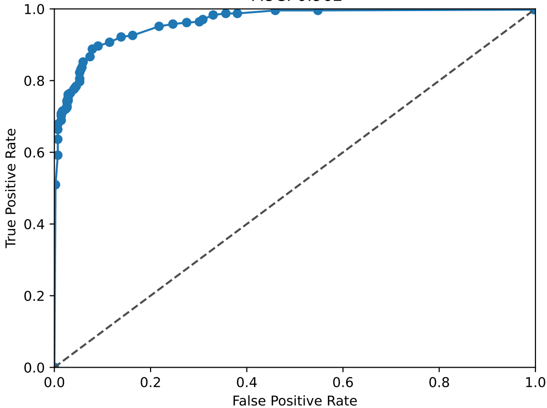
NFKB1 ROC Curve AUC: 0.962
