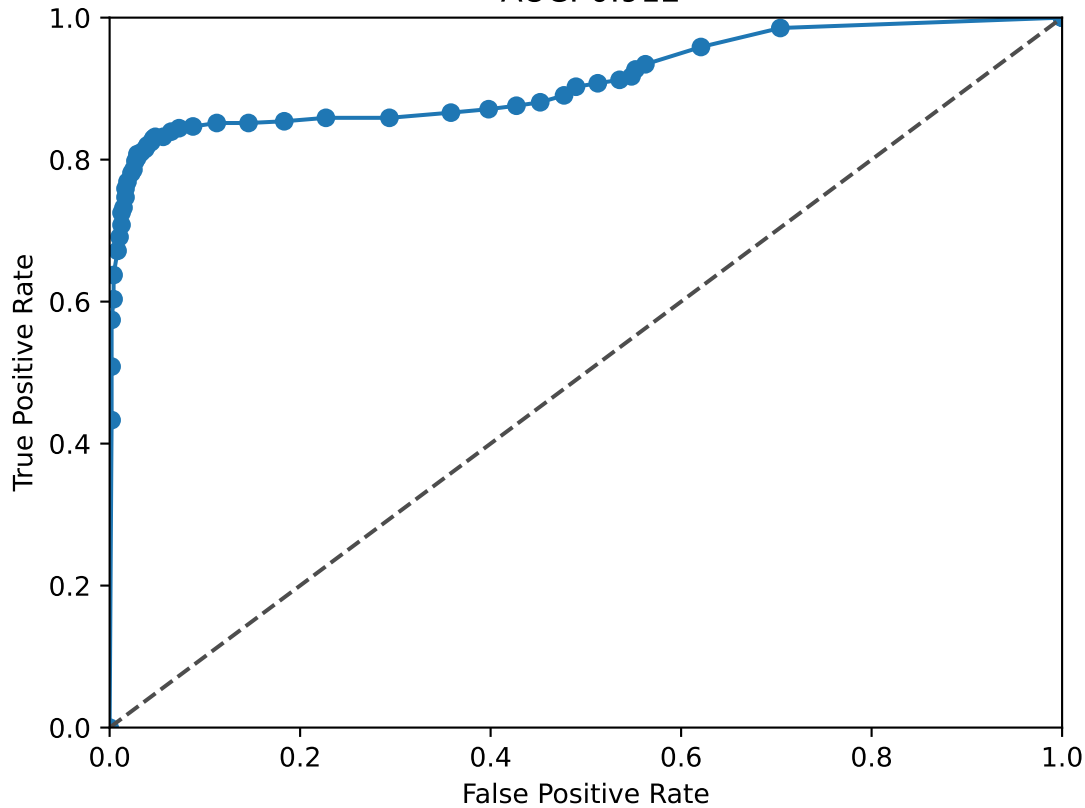
RUNX1 ROC Curve AUC: 0.912
