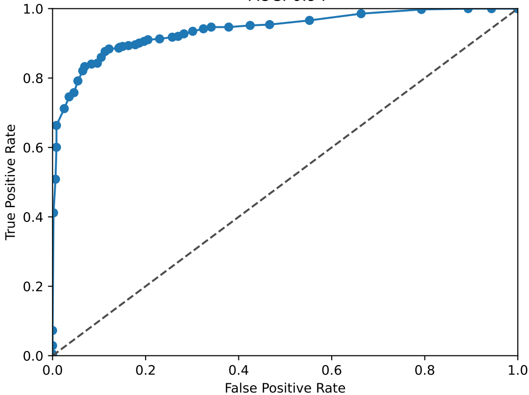
STAT2 ROC Curve
