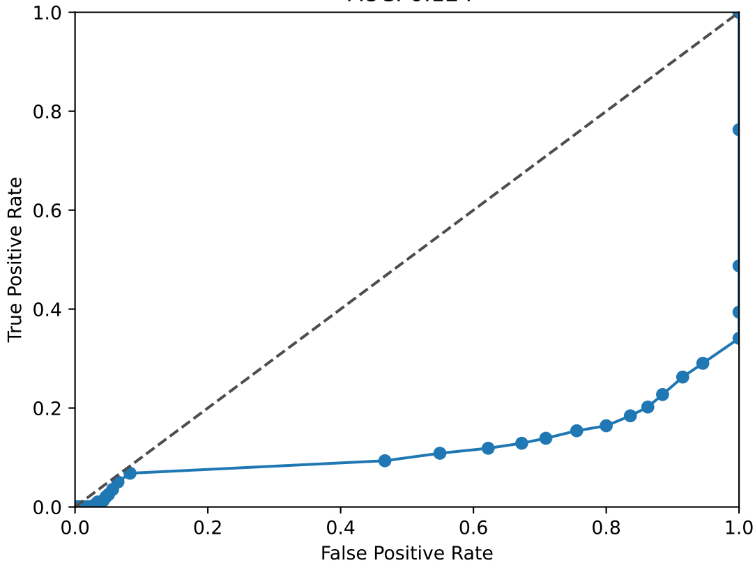
TCF7L2 ROC Curve AUC: 0.124
