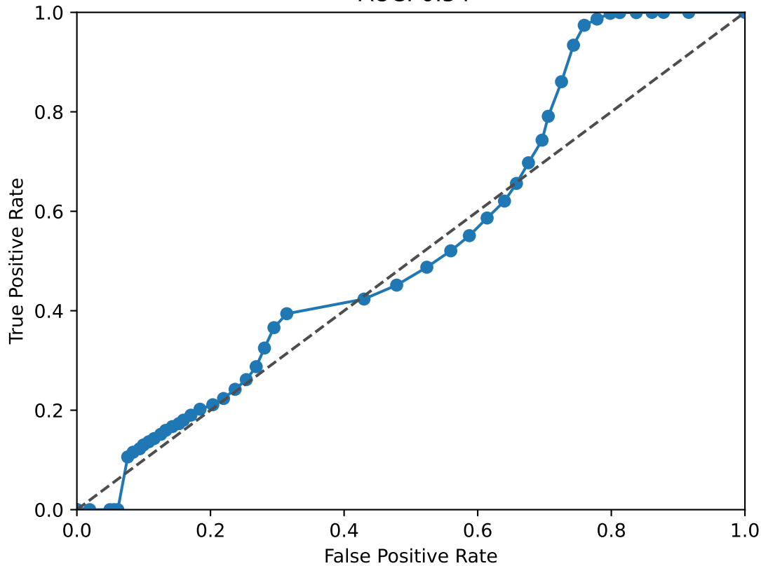
ASCL1 ROC Curve AUC: 0.54
