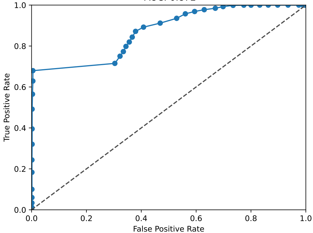
FOS ROC Curve AUC: 0.872
