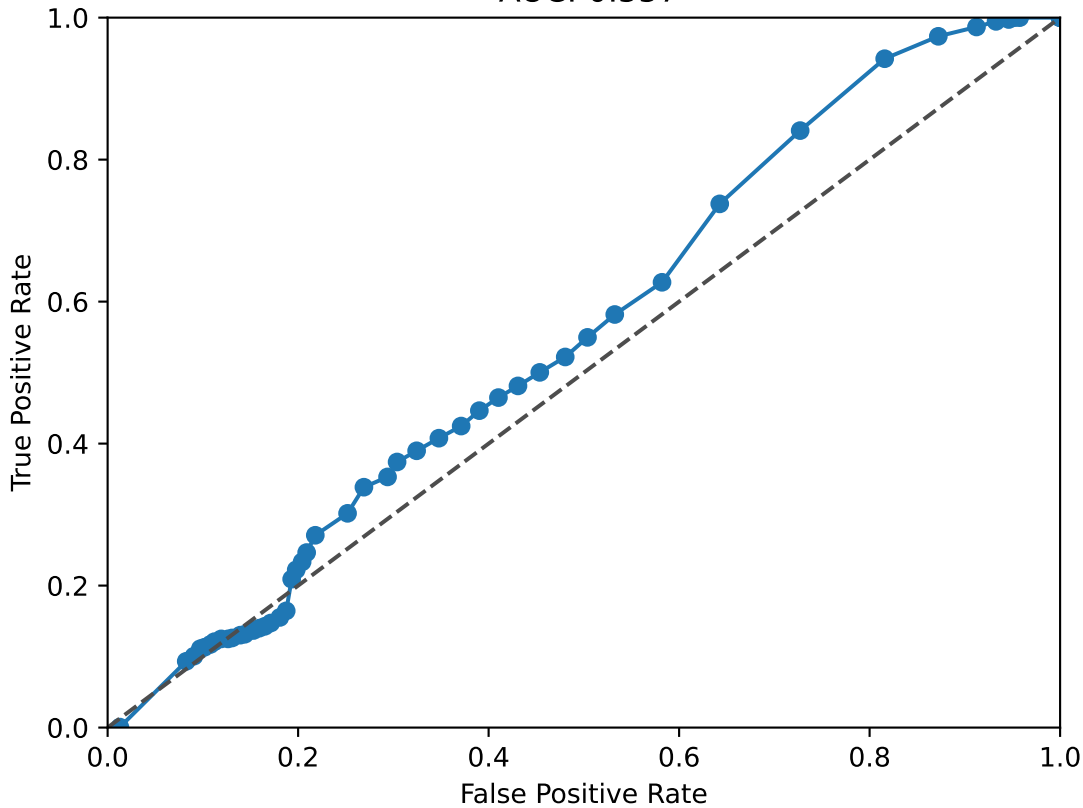
ICAM1 ROC Curve AUC: 0.557
