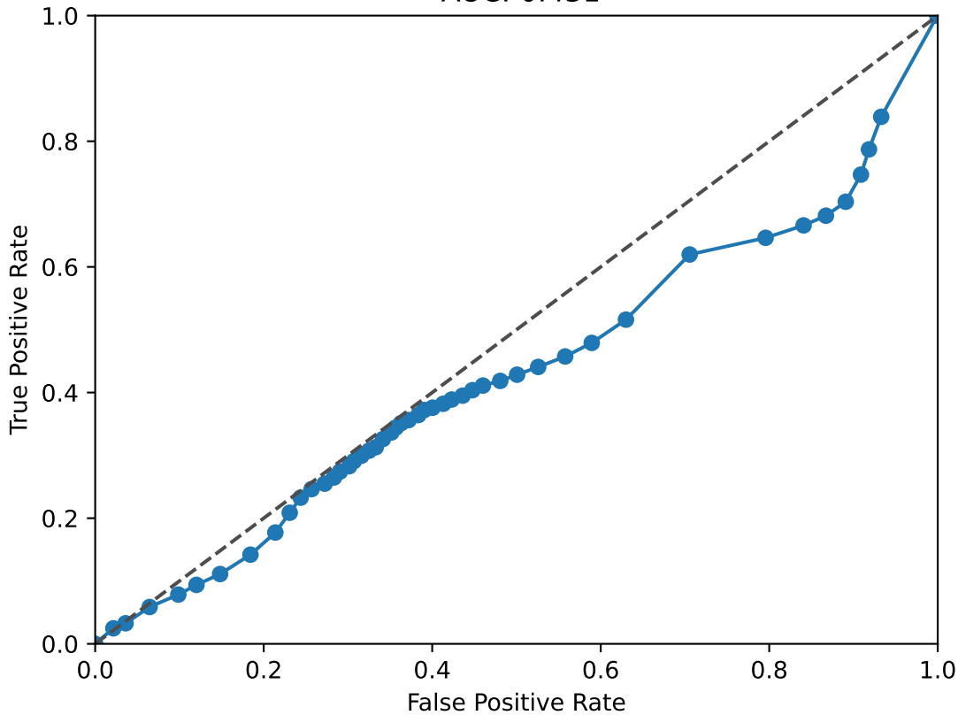
RUNX1 ROC Curve AUC: 0.431
