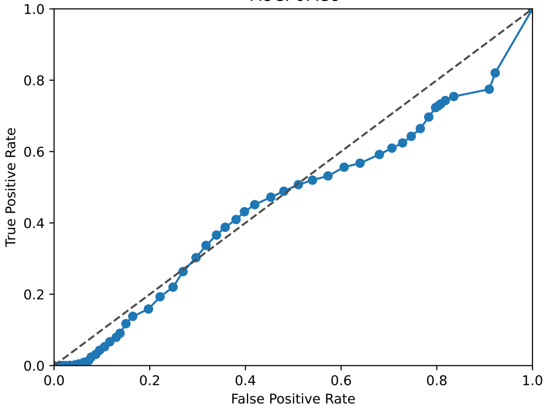
SIX1 ROC Curve AUC: 0.459
