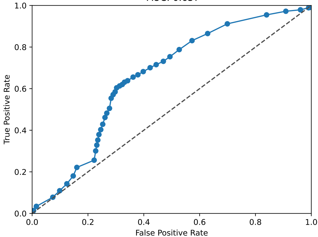
CUX2 ROC Curve AUC: 0.657
