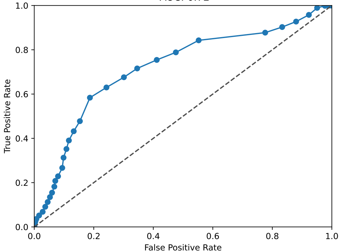
FOS ROC Curve AUC: 0.72
