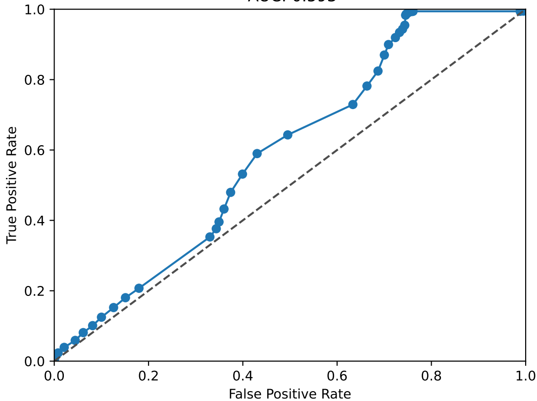
NFATC2 ROC Curve AUC: 0.593
