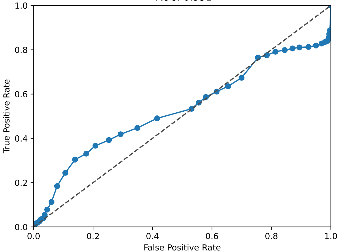
NFIA ROC Curve AUC: 0.531
