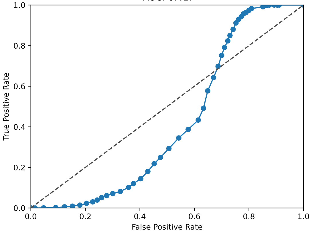
NFIB ROC Curve AUC: 0.417
