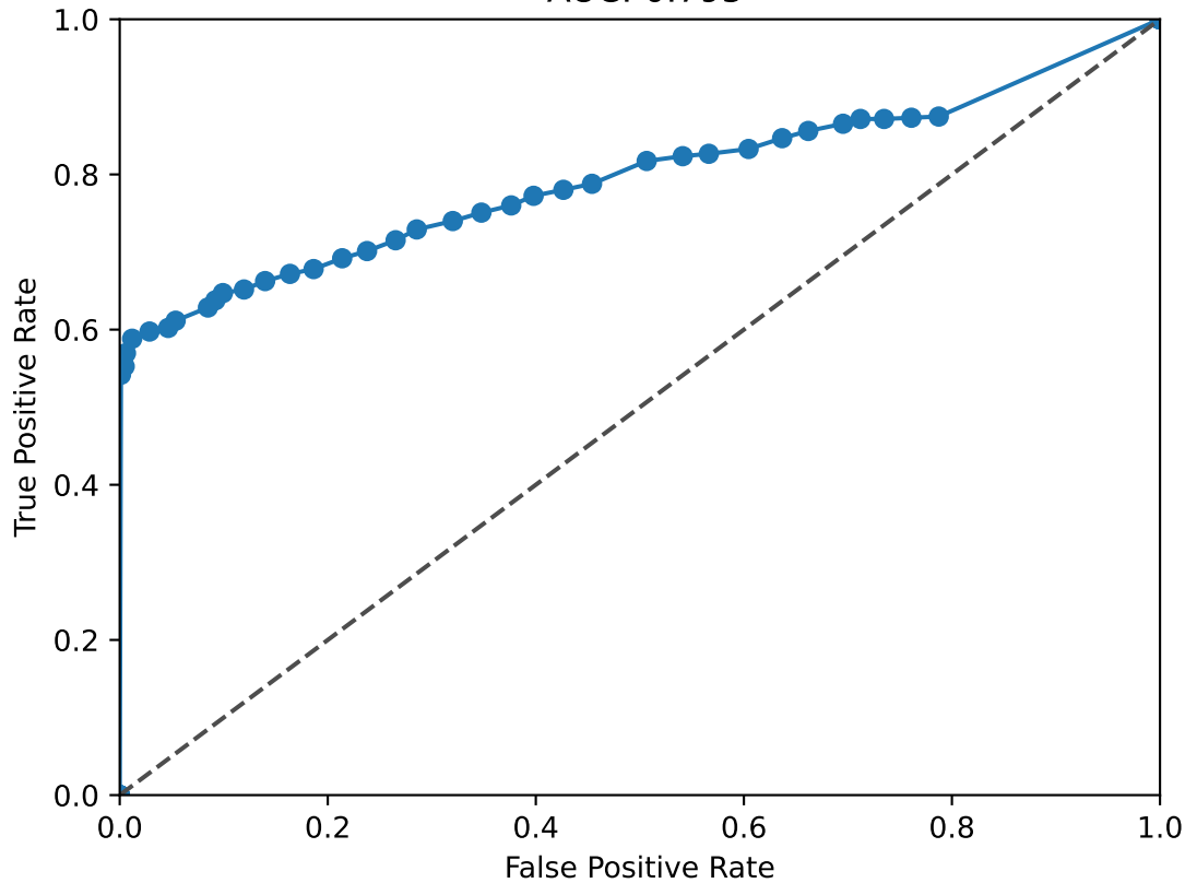
EHF ROC Curve AUC: 0.795
