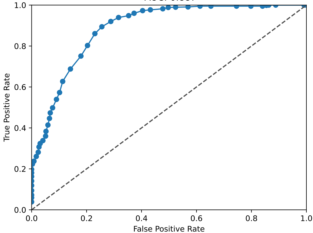
HSF2 ROC Curve AUC: 0.887
