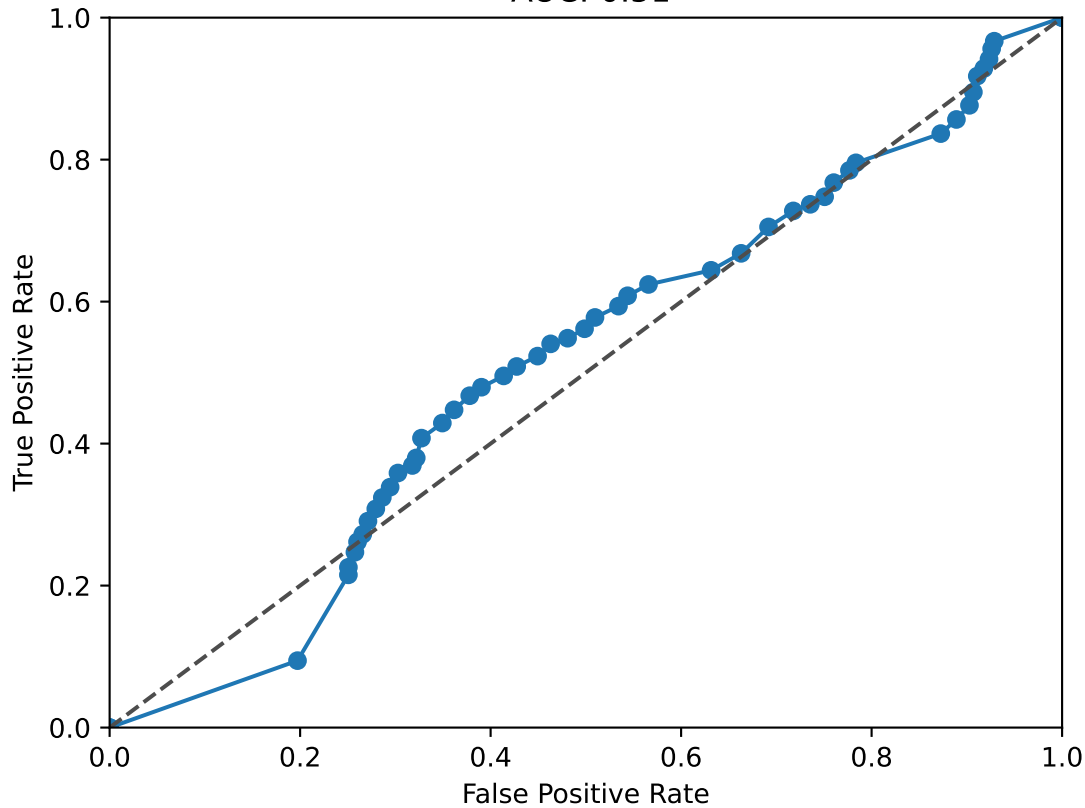
NFKB1 ROC Curve AUC: 0.51
