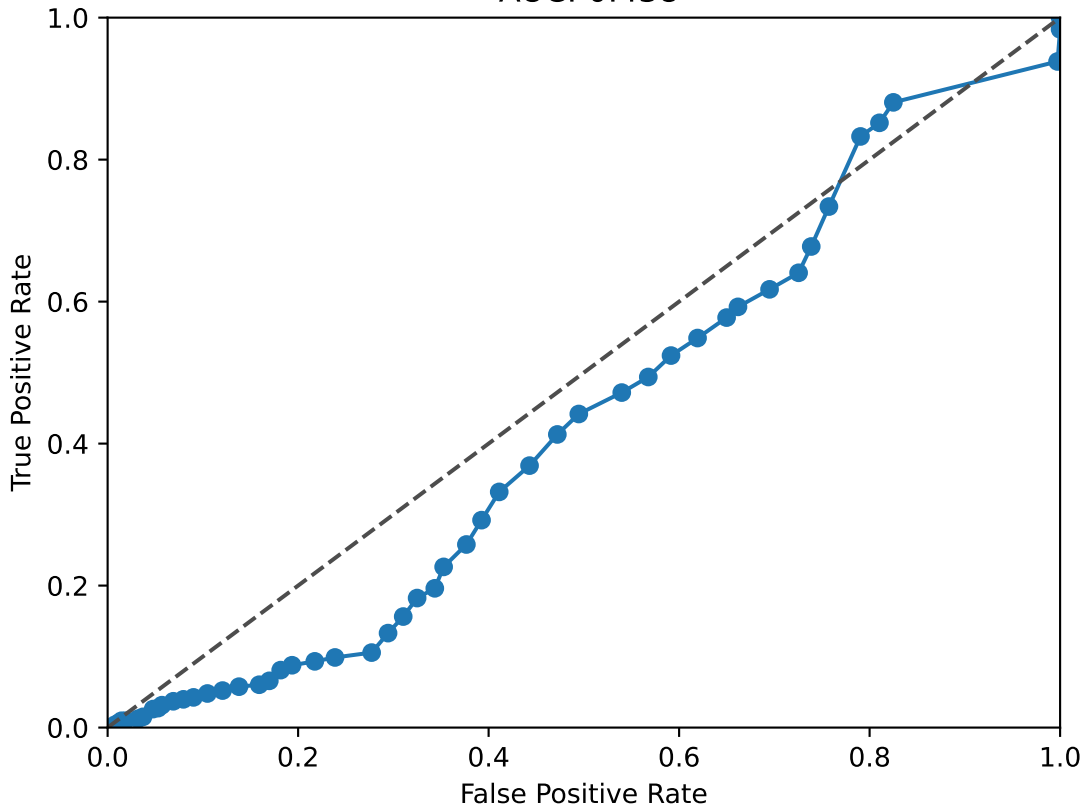
SIX1 ROC Curve AUC: 0.438
