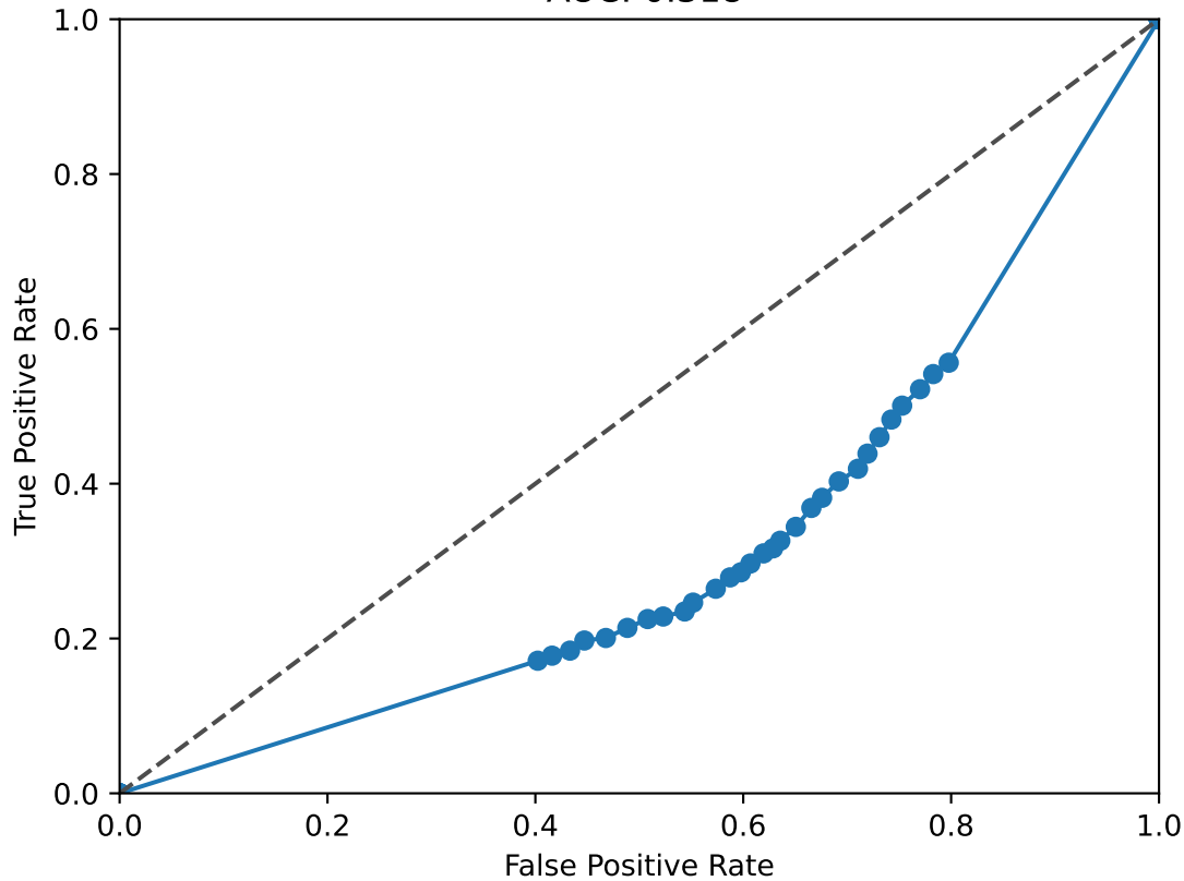
THRB ROC Curve AUC: 0.318
