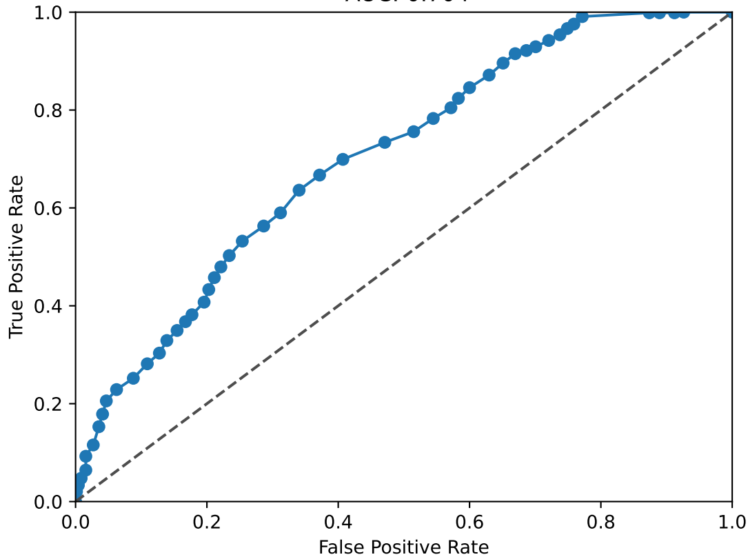
ZBTB20 ROC Curve AUC: 0.704
